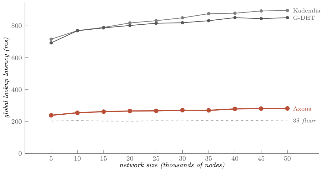
Figure 6: Global lookup latency versus network size at every 5,000 from 5,000 to 50,000 nodes ( 10\times scaling), plotted against the Dabek 3\delta analytical floor (gray dashed). Kademia climbs from 716 to 896 ms as the \log\text{-}N hop tax compounds; G-DHT tracks Kademia almost identically on global lookups (the geographic prefix only helps regional cells). Axona hugs the floor in a tight 239–282 ms band across the whole range ( 1.17\text{--}1.38\times the 3\delta floor) and is essentially flat from 15,000 nodes onward — adding 35,000 more nodes raises latency by 20 ms total. All success rates 100%. Data: sim v0.93.0 / @axona/protocol v1.1.3, May 2026.
